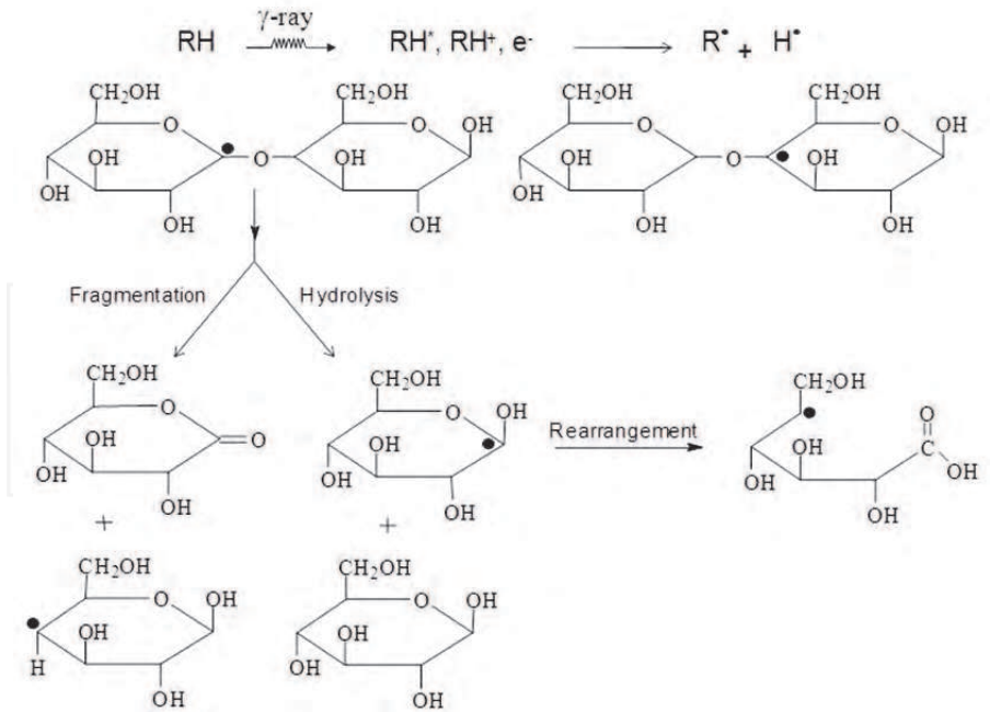
Fig. 12. Events in solid state radiation of hydrocolloids; the glycosidic bond cleavage and chain scission of cellobiose upon solid state radiation of hydrocolloids.
